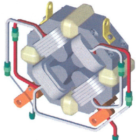
Figure 4. NESTOR quadrupole magnet.
