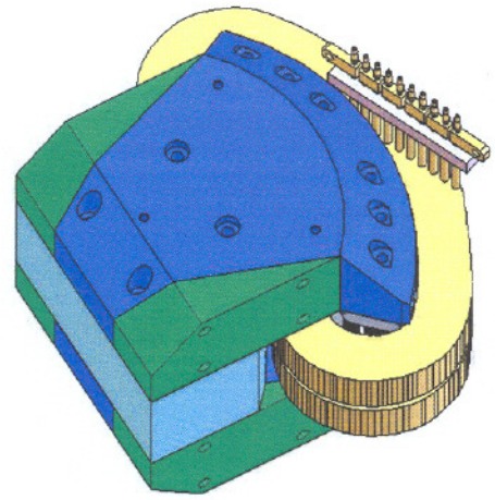
Figure 3. NESTOR bending magnet after reconstruction.
