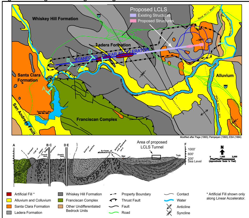
Figure 12. Regional Geologic Setting
