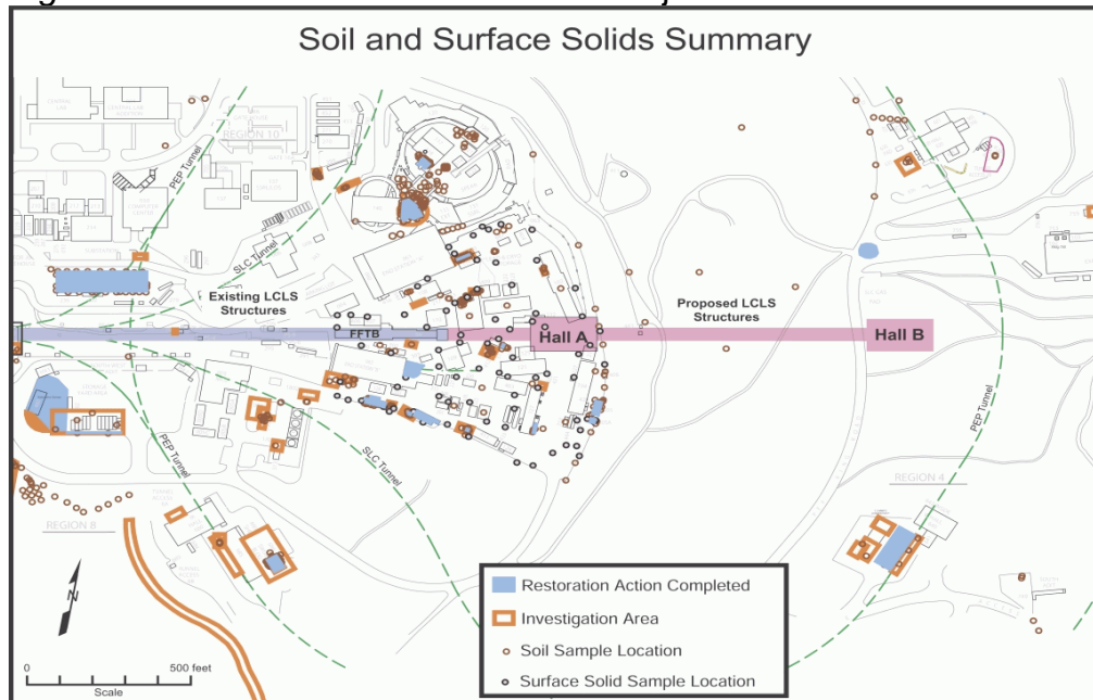
Figure 15. Soil Conditions at the LCLS Project Area
