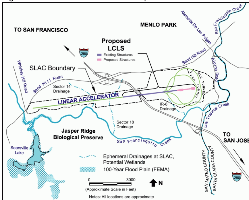
Figure 14. Location of 100-Year Floodplain and Potential Wetlands
