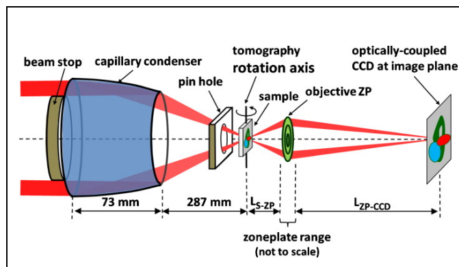
Figure 1. TXM setup. Monochromatic x-rays are focused onto the sample using a capillary condenser. The sample stage is capable of three-axis translation, and rotation for tomography. For XANES imaging the focal length of the zoneplate objective lens is varied over the investigated energy range. Images are captured using a high resolution charge-coupled device (CCD) system. (Figure adapted from Nelson et al. 2011)
