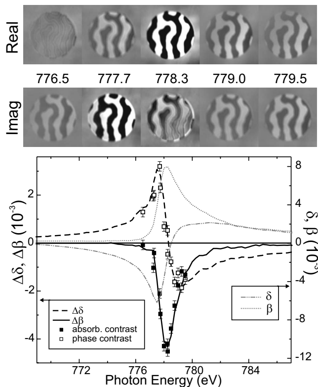
FIG. 4. Top: real (top row) and imaginary (bottom row) parts of the complex real space object image obtained from the holographic difference between left and right circularly polarized x rays as a function of photon energy across the L_3 edge. Bottom: photon energy dependence of the optical constants \delta (dashed-dotted) and \beta (dotted) and the differences \Delta\delta (dashed) and \Delta\beta (solid) of the two polarizations. Spectra are provided by Kortright et al. (Ref. 19). Data points are taken from the image contrast.
