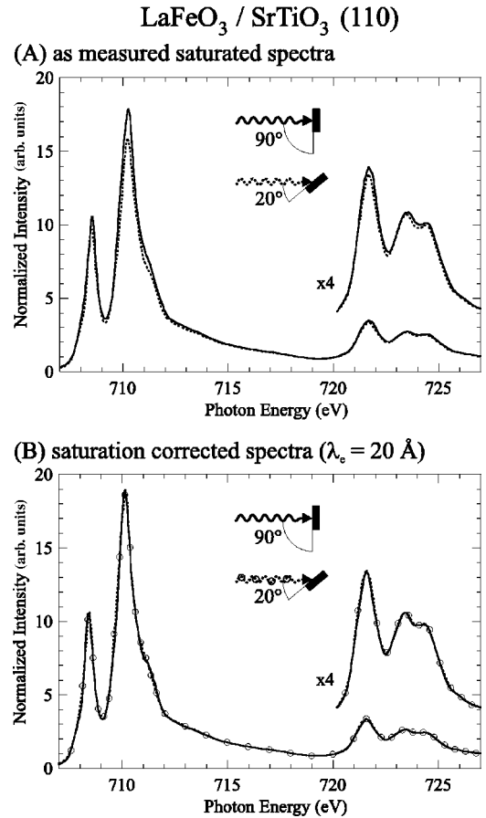
FIG. 5. (A) Normalized total electron yield spectra of LaFeO 3 /SrTiO 3 (110) measured with the same in-plane orientation of the electric field vector in normal (black) and grazing (dashed) incidence geometry [polarization corrected (Ref. 23)]. The differences in peak heights and spectral shapes are due to saturation effects in the electron yield measurements. (B) The same spectra as in (A) corrected for saturation effects as discussed in the text using \lambda_c = 20 Å.
