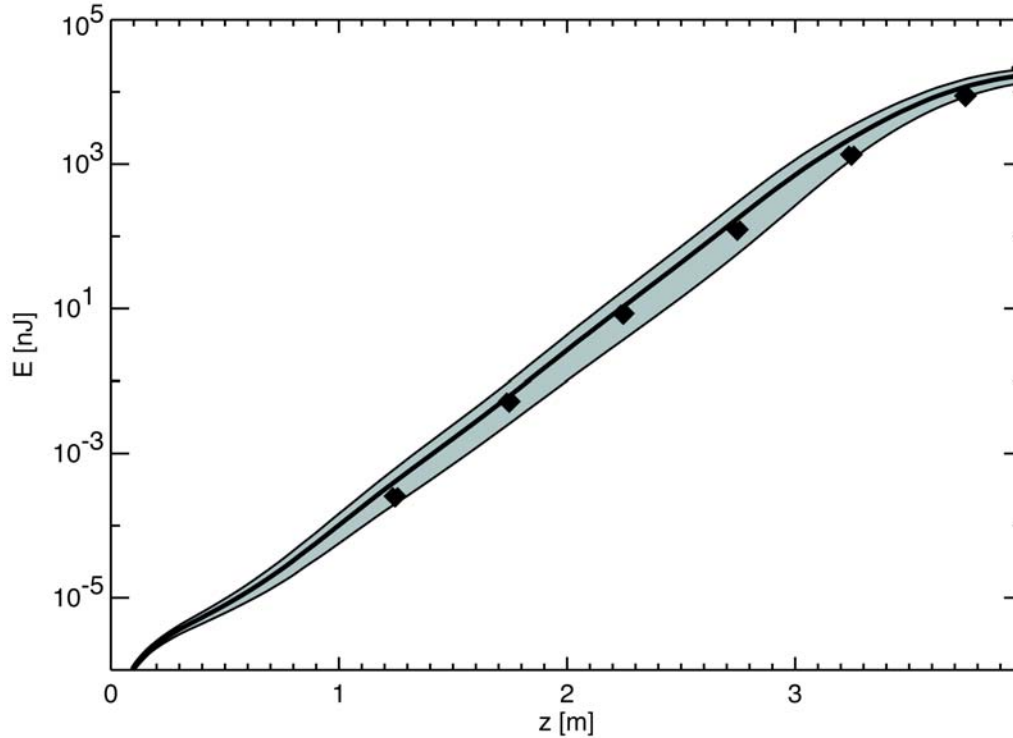
Figure 4. Energy vs. Distance. GENESIS simulation compared to measured data different that in Fig. 1. Gray area indicates a one sigma shot noise fluctuations due to different seedings in GENESIS.
