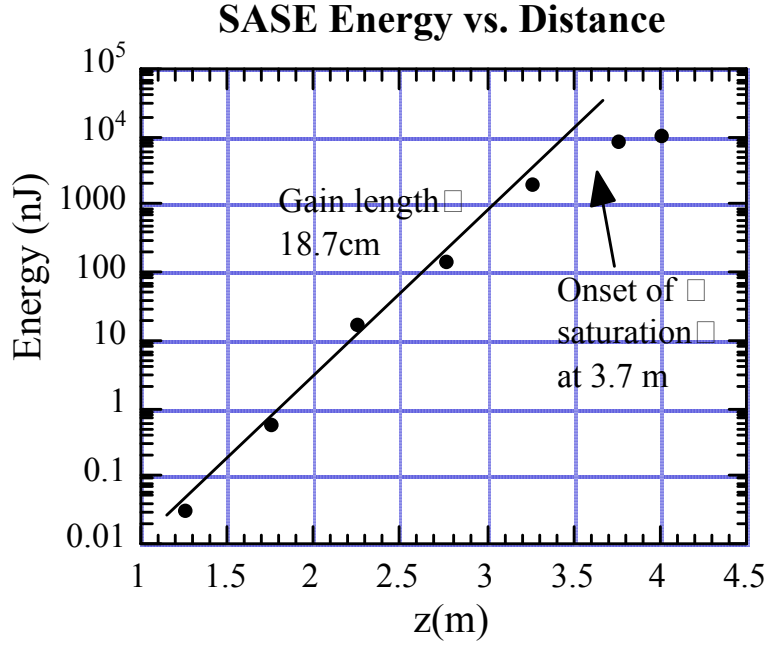
Figure 1. SASE Energy vs. Distance. Deviation of last two points from the line fit of the previous five is evidence that the system is in saturation.
