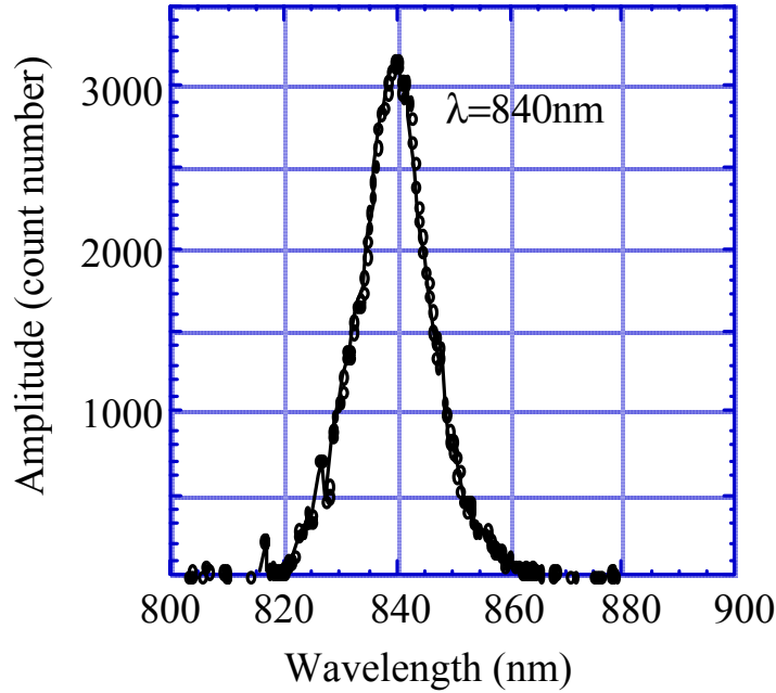
Figure 2. VISA single shot spectrum at saturation. The central wavelength is 840 nm, and the one spike indicates a bunch length of the order of the cooperation length.
