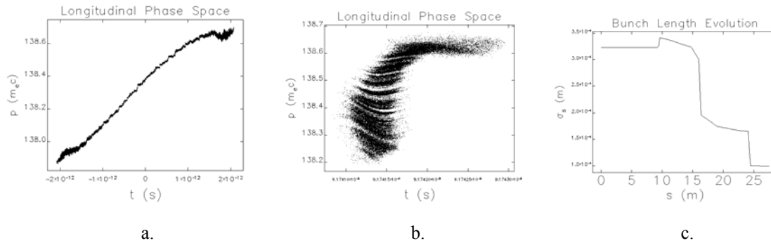
Figure 3. Compression through the dispersion section. 3a. Energy chirped electron beam exiting the linac section, before the dispersion section. 3b. Compressed beam after dispersion section, before the undulator. 3c. Longitudinal beam size from the linac to the undulator.
