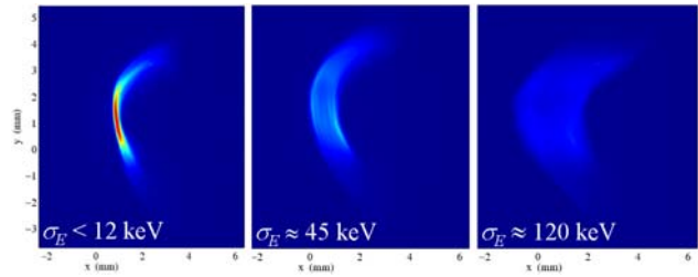
Figure 4: Measured time-sliced energy spread on “YAGS2” screen (see Figure 2) at 135 MeV with laser heater OFF (left), IR laser energy at 40 \mu\text{J} (center), and again at 230 \mu\text{J} (right). The rms energy spread values above agree with calculations.
