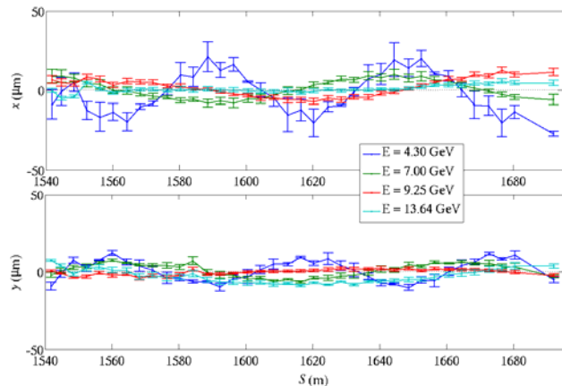
Figure 9: Undulator x (top) and y (bottom) trajectories at four different electron energies (4.3, 7.0, 9.25, and 13.6 GeV) showing the trajectory is highly dispersion-free and well aligned.
