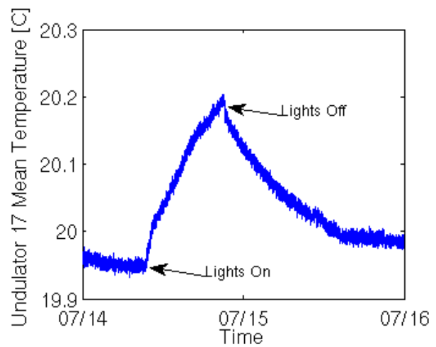
Figure 4: Undulator temperature response to thermal transients caused by turning the lighting on and off.
